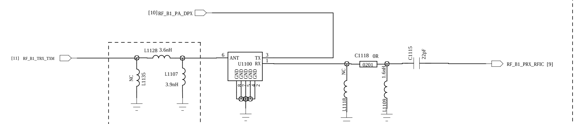
B1 TRX
